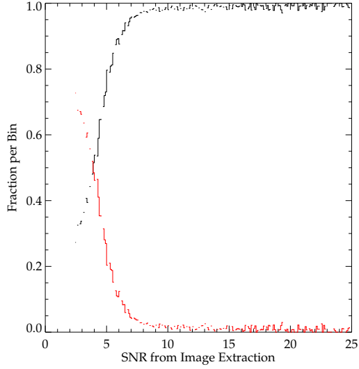
Figure 17: Reliability of image extracted sources under the assumptions given in Section 4.3.3.
