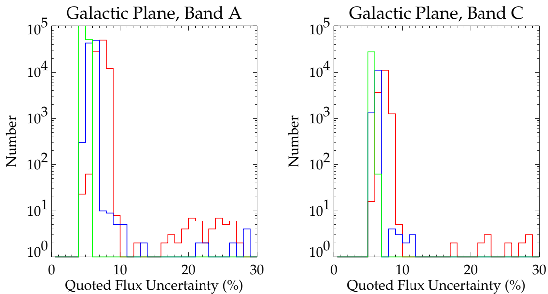
Figure 6: Quoted 1\sigma flux uncertainties for Bands A and C.
