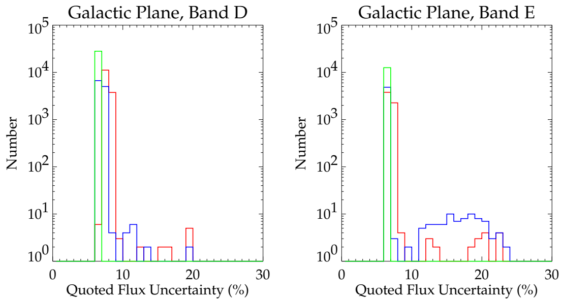
Figure 7: Quoted 1\sigma flux uncertainties for Bands D and E.
