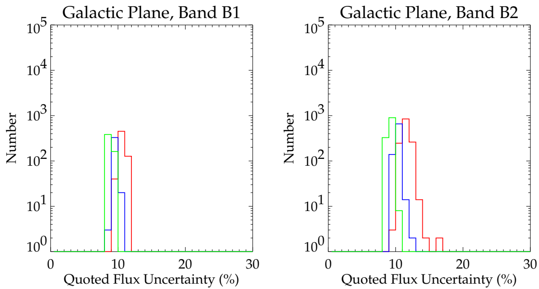
Figure 5: Quoted 1\sigma flux uncertainties for Bands B_1 and B_2 .
