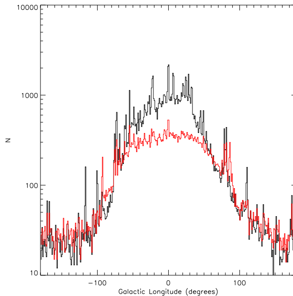
Figure 45: Source density between |b| < 0.5^\circ for PSC V2.3 (black) and PSC V1.2 (red). Longitude bins are 1 degree, therefore bin totals are sources per square degree.
