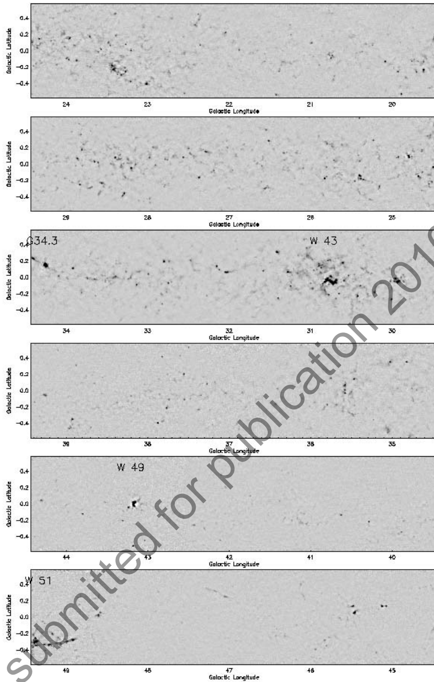
FIG. 19B. l = 19.5 to l = 49.5 . G34.3+0.15, W 51, W 43, W 49, and M 17 appear to be saturated, but this is only a display artifact. The 20 < l < 40 region through the 4-8 kpc molecular ring and approximately the termination of the galactic bar is particularly rich in clumps.
