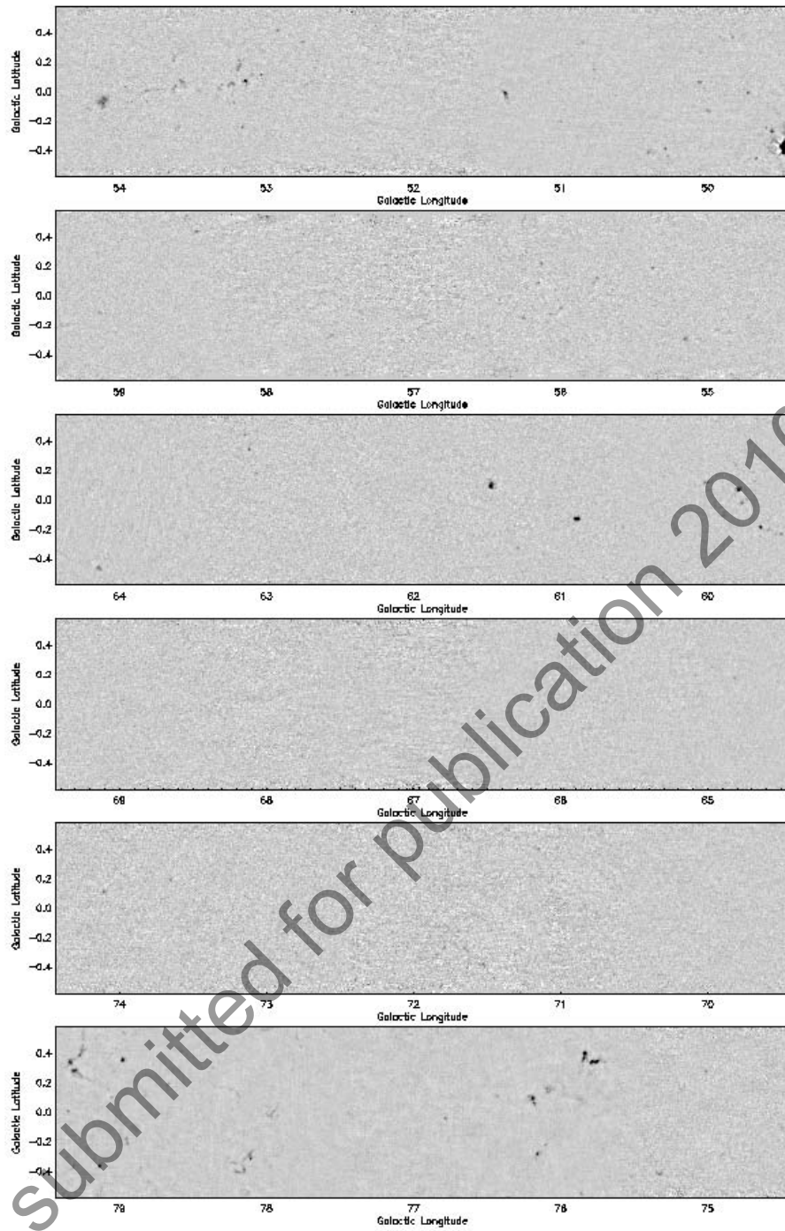
FIG. 19C. — l = 49.5 to l = 74.5 . In comparison to the inner galaxy, the 65 < l < 75 has a very sparse population of faint clumps.
