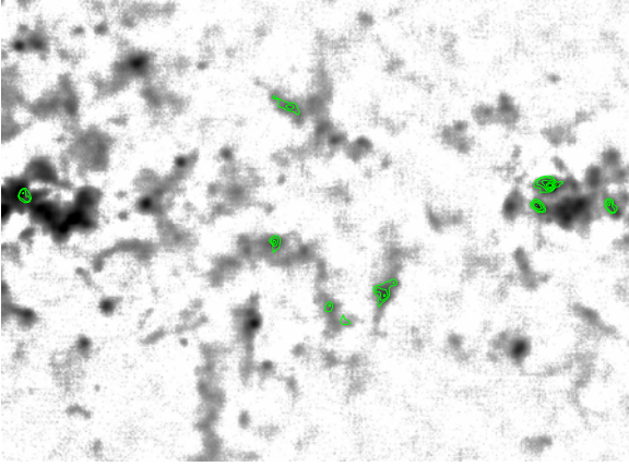
(a) Left: the Bolocam map in a portion of the l = 30 field. Right: the SLC maps in the same region. The green contours on the Bolocam map indicate the positions of the SLC sources. Note that the SLC maps only cover a small portion the entire region shown, corresponding to the isolated sources indicated by the contours. Negative bowls in both images are forced to zero before cross-correlating.
