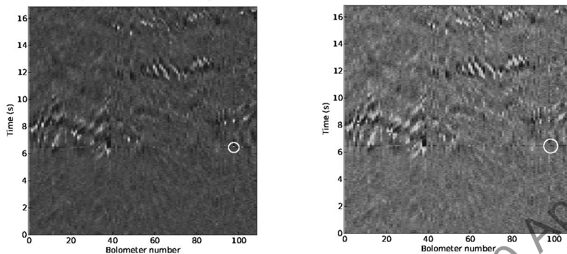
FIG. 9.— An illustration of the flagging process using the waterfall plot. Left: The glitch whose time series is shown in Figure 8 is circled in the waterfall plot (bolometer 98, around 6.2s). It appears as a single hot pixel. Because of the PCA subtraction, the effect of the glitch also propagates over the other bolometers, appearing as a horizontal stripe. Right: The same data displayed with the time point including the glitch flagged out and rescaled. The other features in the plot correspond to passages of the bolometers over real emission, including NGC 7538, which has a peak of \sim 7 \text{ Jy beam}^{-1} .
