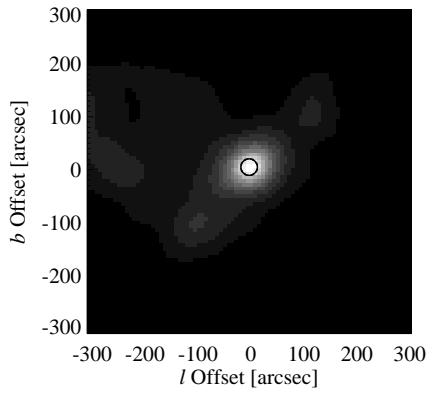
(b) The cross-correlation map of the BGPS and SLC maps in Figure 5(a).
