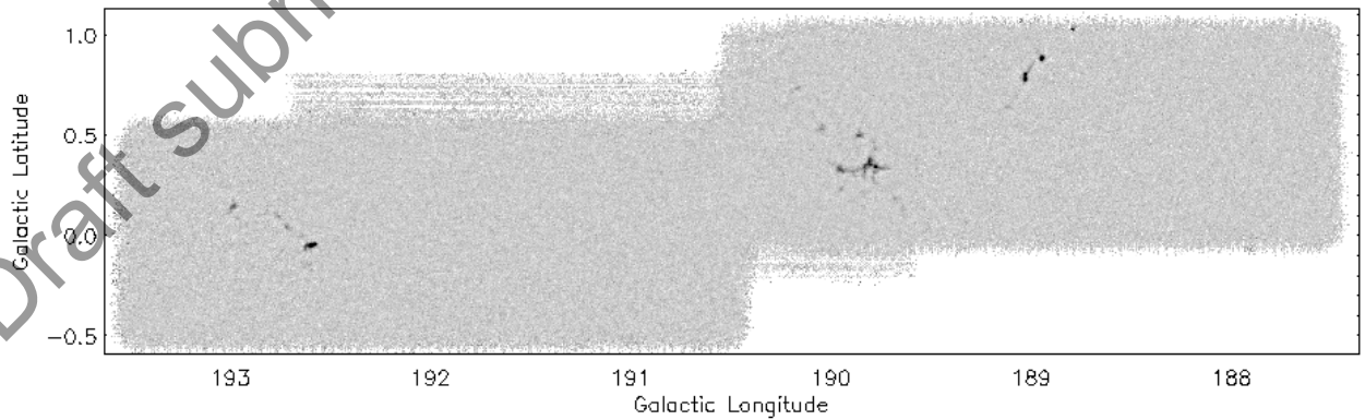
FIG. 19i.— Gem OB1. This region has been thoroughly surveyed in \text{NH}_3 , and is discussed in Dunham et al. (2010).
