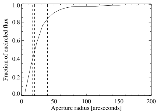
FIG. 14.— Left: The radial profile (solid) of the Bolocam PSF derived from Neptune and Uranus observations, including all bolometers. The main lobe is well approximated by a Gaussian (dotted) and the sidelobes are due to the Airy pattern from truncation of the beam at the cold Lyot stop (dashed). Error bars indicate the azimuthal standard deviation. Right: Enclosed flux in an aperture of a given radius based on the measured PSF. This curve is the basis of the point source aperture corrections.
