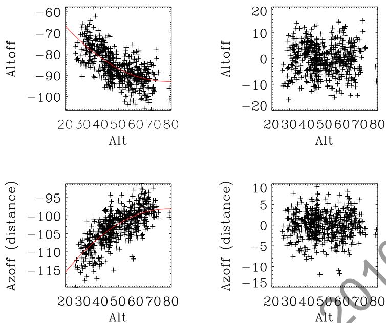
(a) The pointing model for Epoch V, from which the master reference images were derived for subsequent alignment. The left column is the pointing model correction and the right the residuals (both in arcseconds). The red line indicates the fitted model. 510 pointing sources were included, and the final RMS was 5.77'' in altitude and 3.21'' in azimuth, or a total RMS offset of 6.6'' . No systematic offset with azimuth was found.
