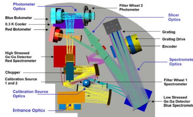
Optical layout of the PACS instrument
