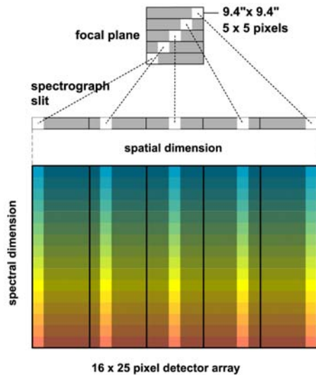
Projection of focal plane onto spectrometer arrays
