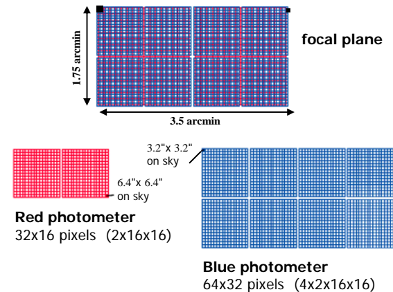
Projection of focal plane onto bolometer arrays
