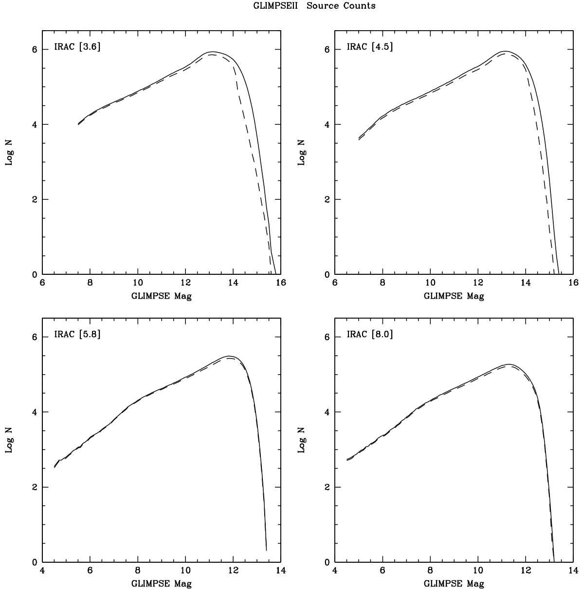
Figure 2: GLIMPSEII source counts versus magnitude. Plotted is the logarithm of the source counts in the GLIMPSEII Catalog (dashed lines) and Archive (solid lines) binned every 0.1 magnitudes. Each of the 4 bands is plotted, showing the effective limiting magnitude for each band. The band 1 & 2 distributions are very similar since most sources that make it into the Archive or Catalog have data in those bands. Sources from the entire GLIMPSEII region were used in these plots.
