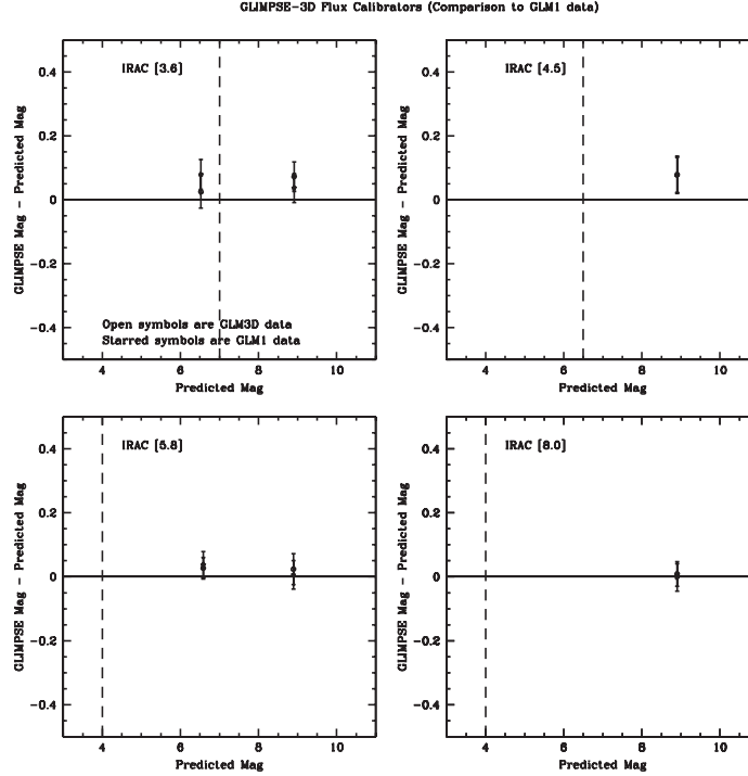
Figure 4: Comparison of two GLIMPSEI flux calibrators that are in the overlap areas for the three GLIMPSE3D regions of this data delivery. They show good agreement between the GLIMPSEI and GLIMPSE3D extractions as well as agreement to Martin Cohen's predicted magnitudes for each IRAC band. Error bars are the root-sum-of-squares of the errors of both the extracted and predicted magnitudes for each source. The vertical lines are the best estimates of the saturation limits.
