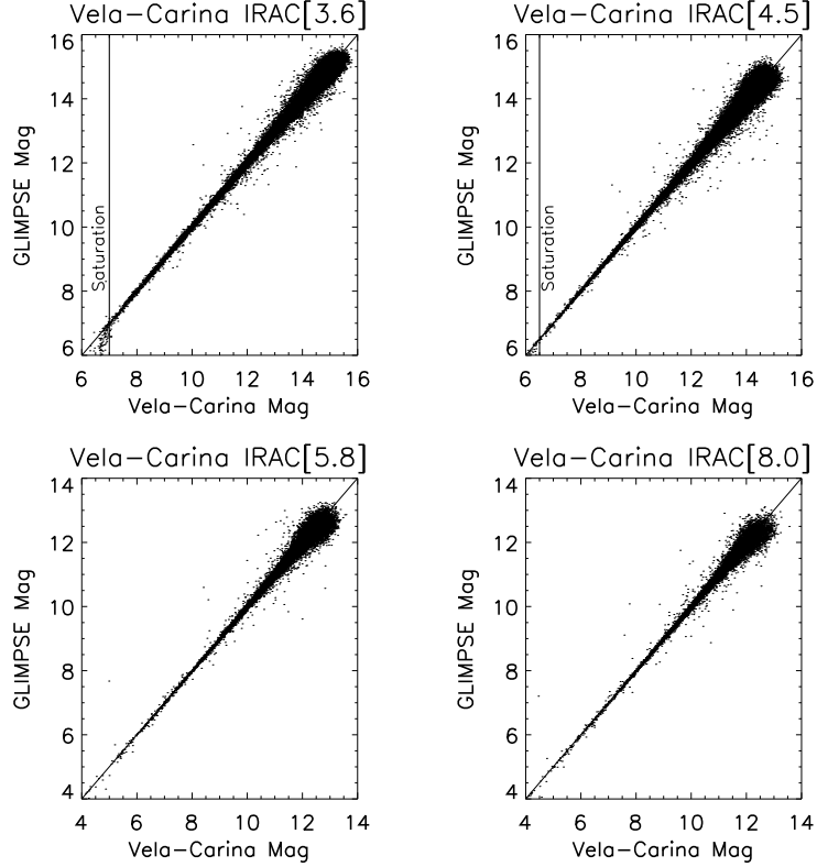
Figure 5: Comparison between overlap regions between Vela-Carina and GLIMPSEI and OSV data. There are about 47263 Vela-Carina sources that overlap the GLIMPSEI area at l=295^\circ and 102845 Vela-Carina sources that overlap the OSV area at l=284.2^\circ . This shows the good agreement between datasets.
