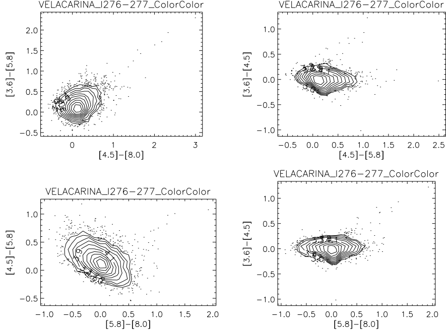
Figure 6: Color-color plots of the region l = 276 - 277^\circ and b = -1.5 to +0.5^\circ for sources in the Catalog. 10 contours are evenly spaced between \log(\# \text{ sources/mag}^2) = 2.0 and the log of maximum number of sources per square magnitude. The contours are labeled with the log of the number of sources per square magnitude. Outside of the lowest contour, the positions of individual sources are plotted.
