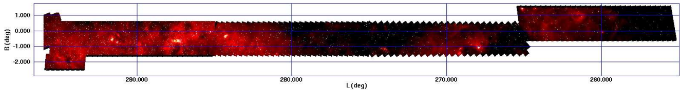
Figure 1: The area observed by the Vela-Carina survey. This is a 3-color image ([3.6], [4.5] and [8.0] in blue, green, and red respectively) of the survey region. Source lists and enhanced images for the entire survey area have been delivered to IRSA.
