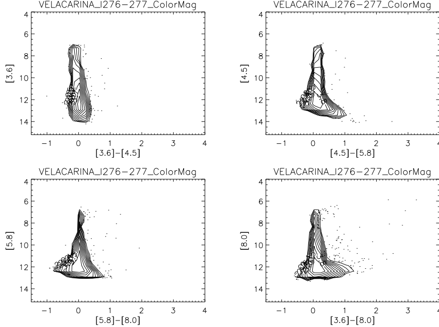
Figure 7: Color-magnitude plots of the region l = 276 - 277^\circ and b = -1.5 to +0.5^\circ for sources in the Catalog. 10 contours are evenly spaced between \log(\# \text{ sources}/\text{mag}^2) = 2.0 and the log of the maximum number of sources per square magnitude. The contours are labeled with the log of the number of sources per square magnitude. Outside of the lowest contour, the positions of individual sources are plotted.
