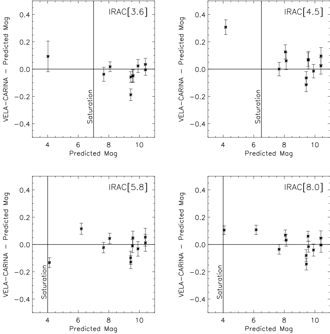
Figure 4: Vela-Carina Flux Calibrators. Comparison of eleven GLIMPSEI and Observation Strategy Validation (OSV) flux calibrators that are in the overlap areas with the Vela-Carina survey. They show good agreement between the GLIMPSEI, OSV and Vela-Carina extractions as well as agreement with Martin Cohen’s predicted magnitudes for each IRAC band. Error bars are the root-sum-of-squares of the errors of both the extracted and predicted magnitudes for each source. The vertical lines are the best estimates of the saturation limits.
