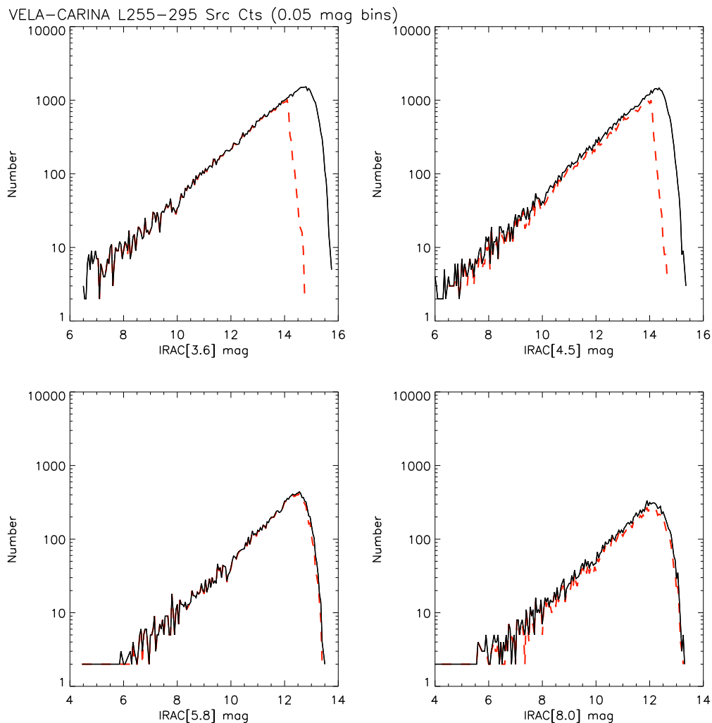
Figure 2: Plotted is the logarithm of the source counts in the Vela-Carina Catalog (dashed lines) and Archive (solid lines) binned every 0.05 magnitudes. Each of the 4 bands is plotted, showing the effective limiting magnitude for each band. Sources from all of the Vela-Carina survey were used for these plots.
