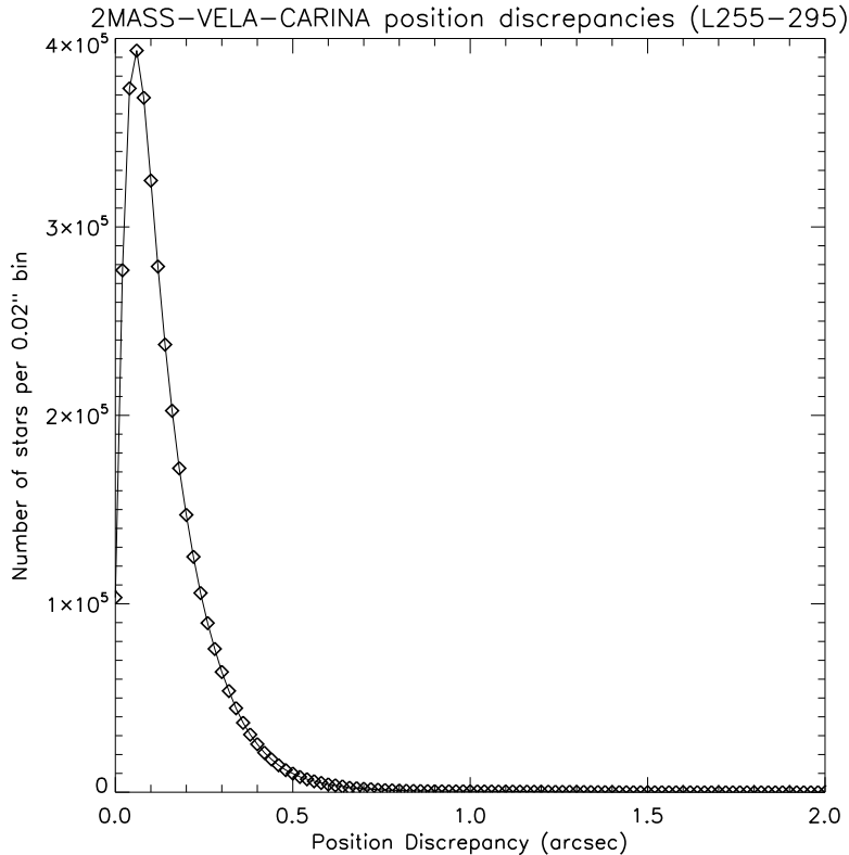
Figure 3: Comparison of Vela-Carina source positions to their corresponding 2MASS PSC positions from all sources in the survey. The astrometric discrepancy plotted is the angular separation in arcseconds between the Vela-Carina position and the 2MASS position. Note that sources with 2MASS associates have Vela-Carina positions that are in part derived from the 2MASS position. Thus this is not a comparison of a pure IRAC-only position with the 2MASS position.
