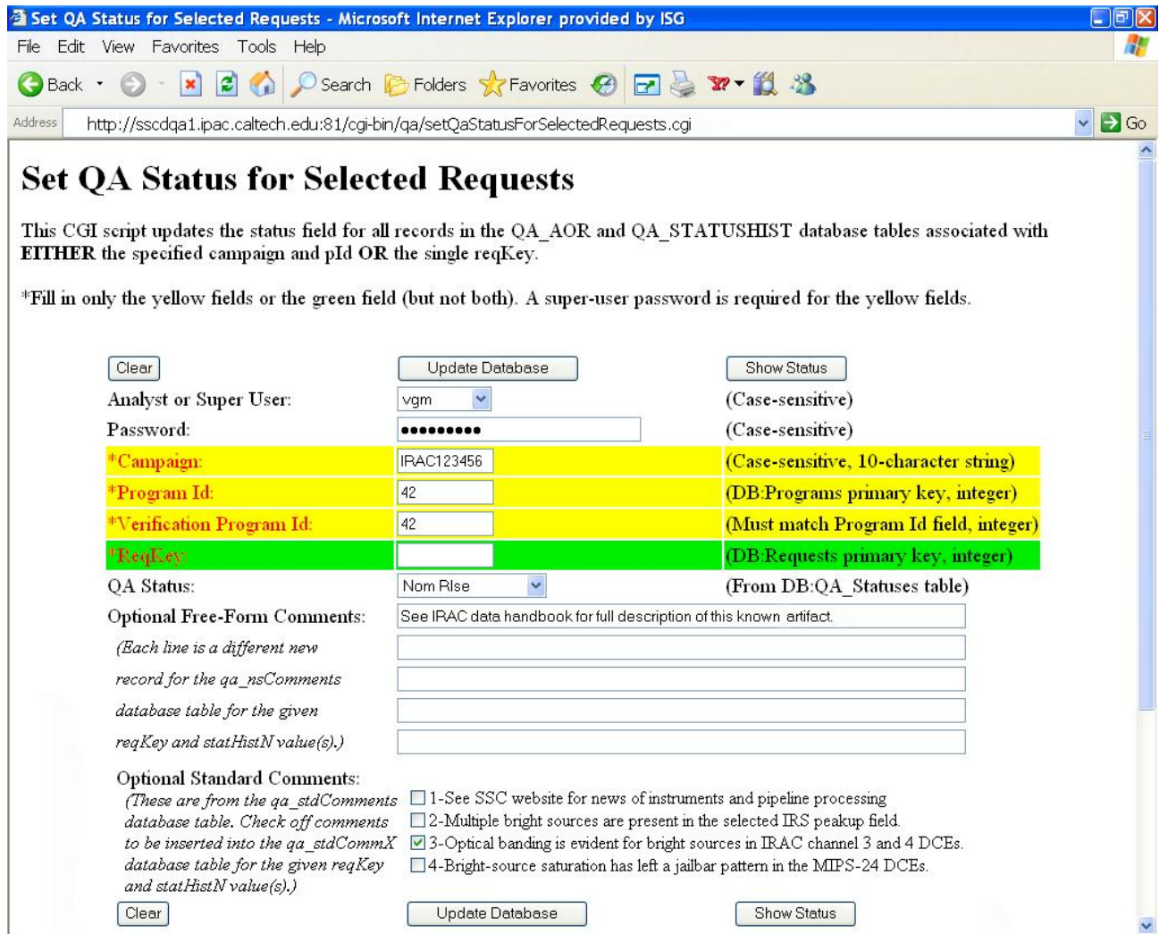
Fig. 3. Screen shot of one of the CGI scripts of the DQA software system at the Spitzer Science Center.
